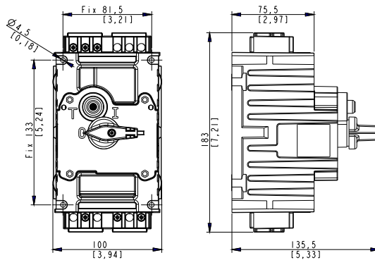
2 Poles Circuit breaker with GFI 2 Poles + Aux Circuit Breaker with GFI
